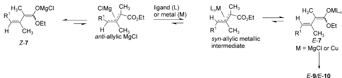
Scheme 3. Possible mechanism for the formation of E - 9 and E - 10 .
