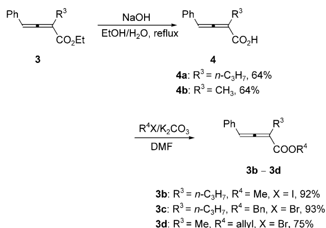
Scheme 2. Synthesis of 2,3-allenoates 3b–3d .
