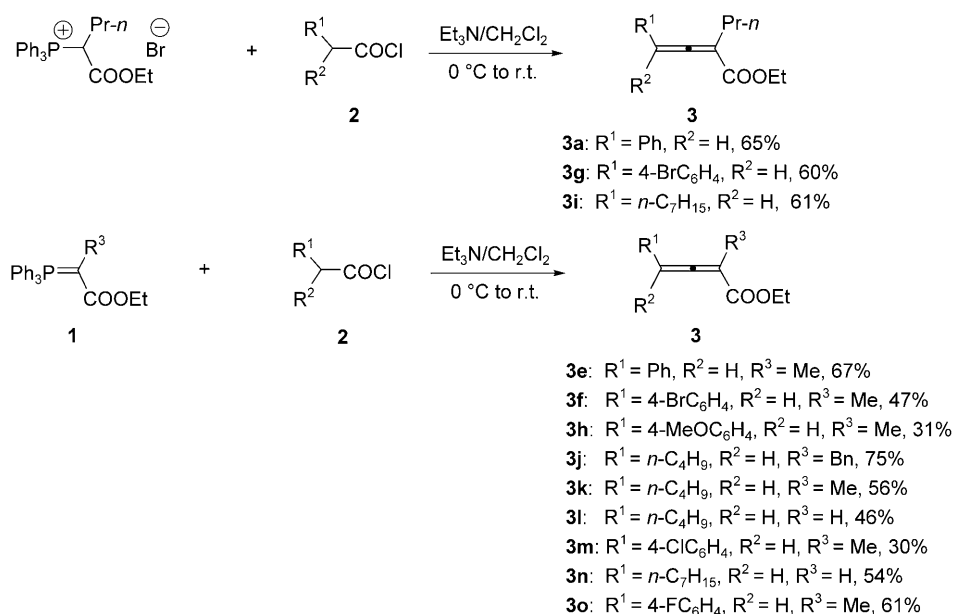
Scheme 1. Synthesis of 2,3-allenoates 3a and 3e–3o .
