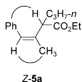
Figure 1. NOE study of Z-5a .
